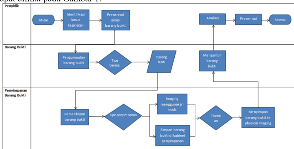
Gambar 1. Alur Kerja Metode Digital Forensic Research Workshop
