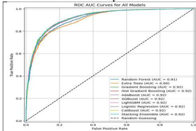
Figure 4. ROC-AUC curves for all models
