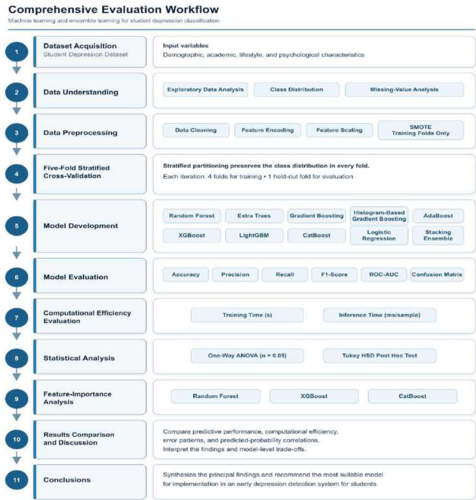
Figure 1. Research workflow for comparing ensemble learning methods in university student mental health classification
