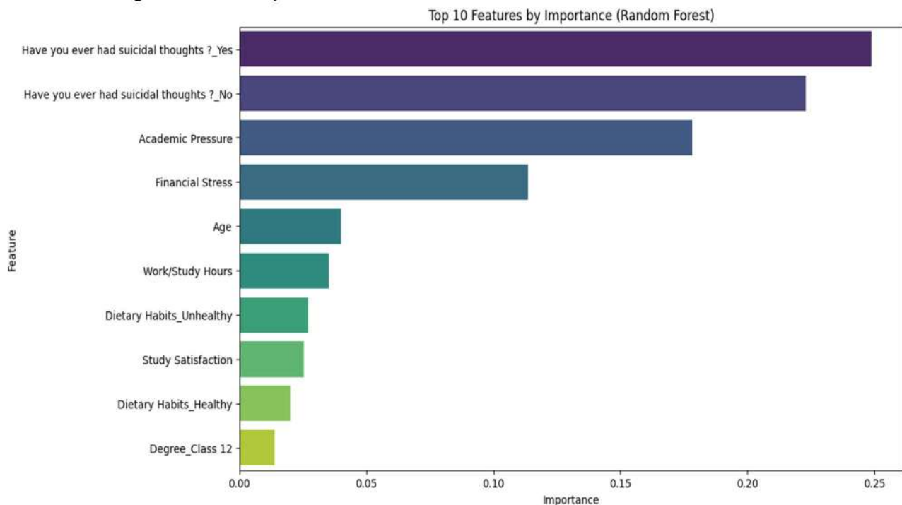
Figure 10. Ten most important features according to Random Forest
