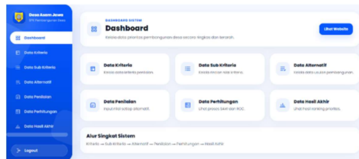
Figure 2. Home Screen
