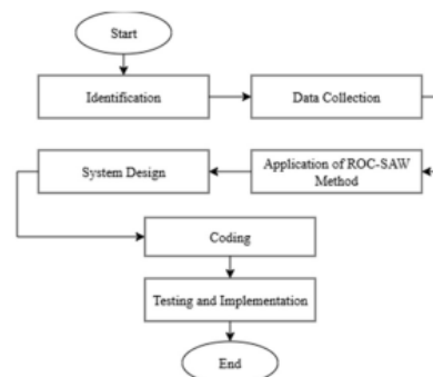
Figure 1. Research Stages
