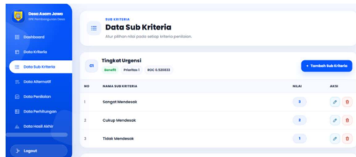
Figure 4. Sub-criteria Page
