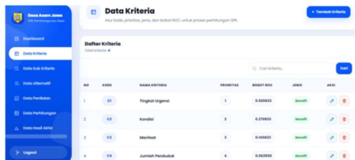
Figure 3. Criteria Page
