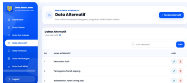
Figure 5. Alternatives Page
